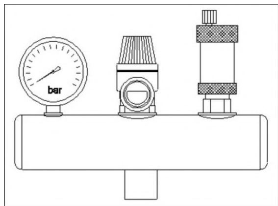
Fig 5. Boiler safety kit
