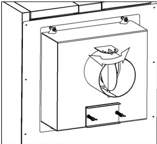
Fig 10. Chimney damper
