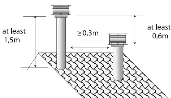
Fig 3. Chimney distances
