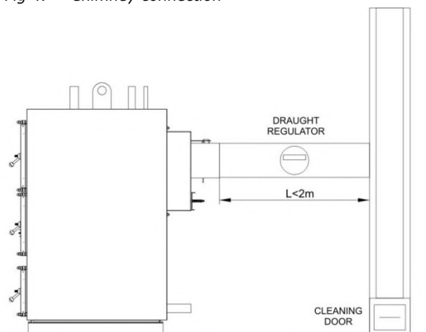
Fig 4. Chimney connection
